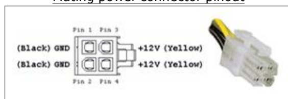
Mating power connector pinout
